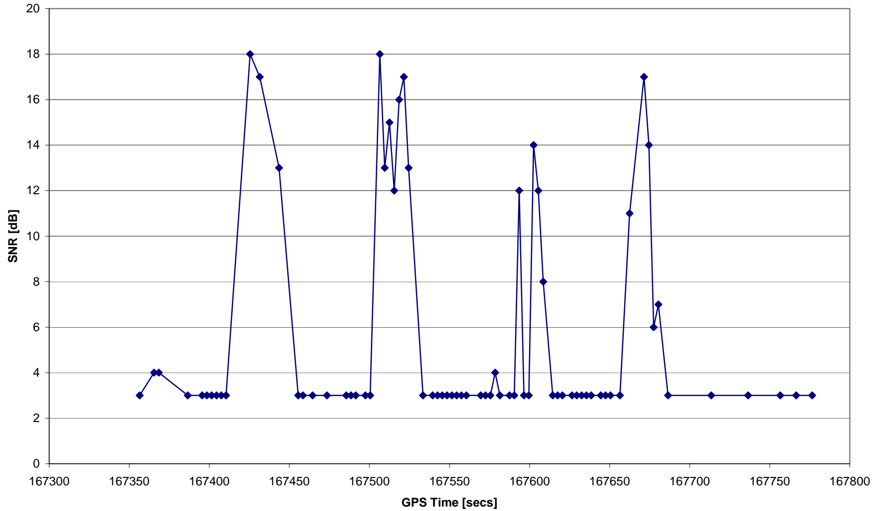
PCsat GPS Receiver SNR for PRN 14 (2002/06/24; GPS Week: 1172)
